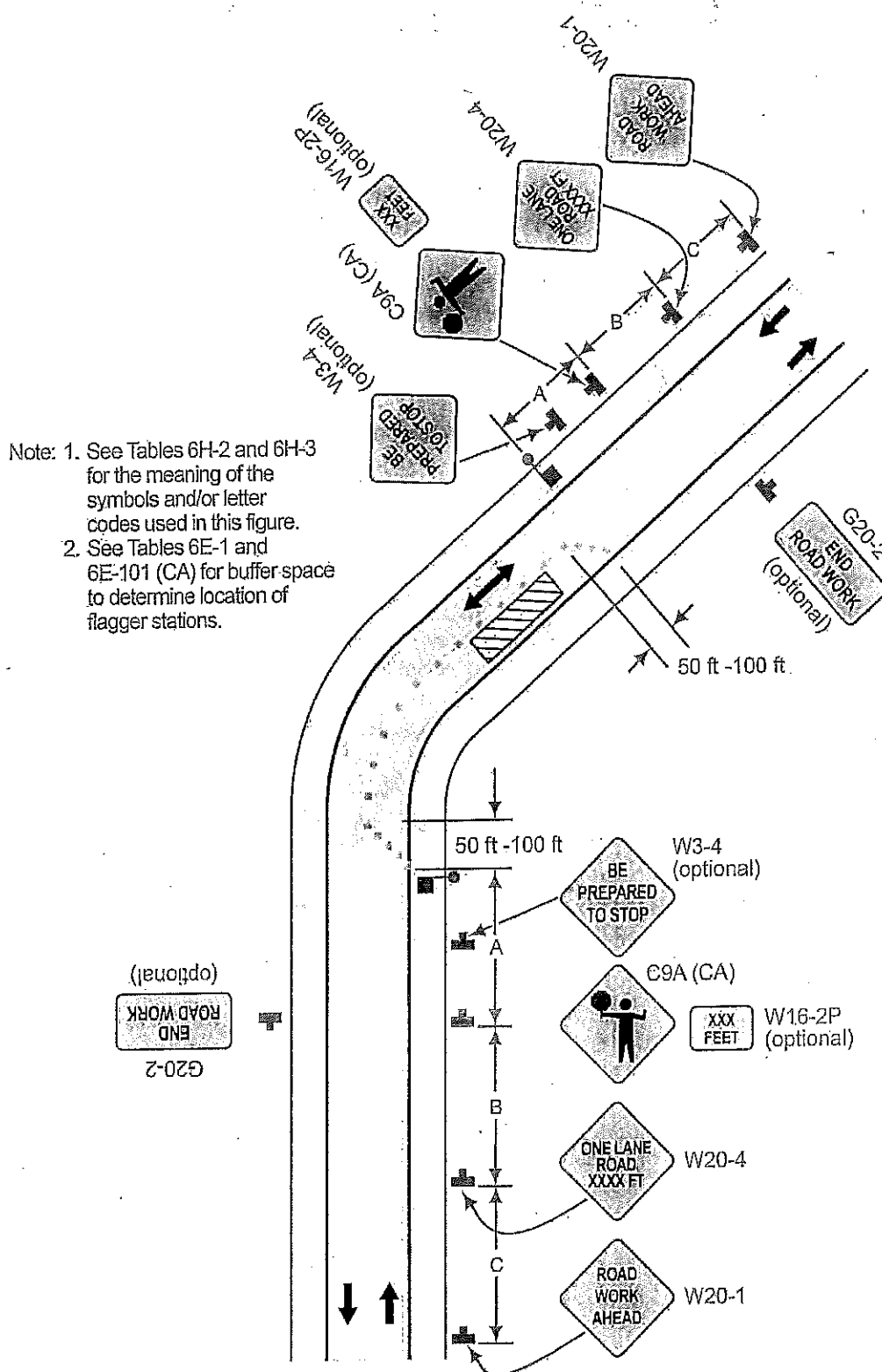
Typical Application 10
